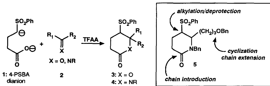
Figure 2. Utility of 4-PSBA - to prepare lactones and lactams and target intermediate.
